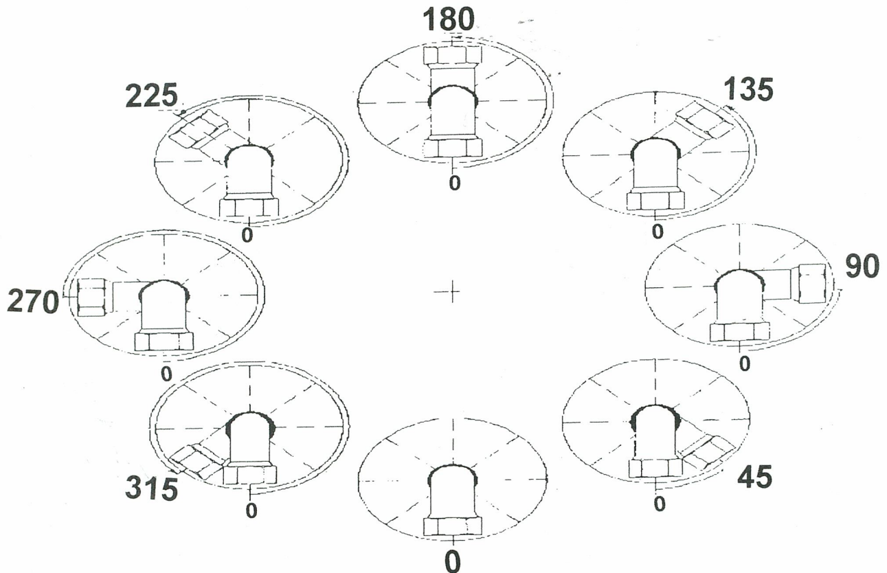
Figure 5.6.1. Offset Angles
